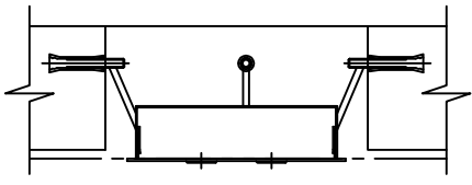
DETAIL OF HALL BUTTON
