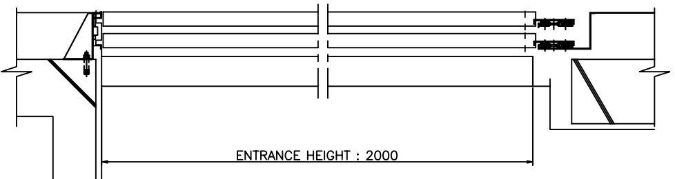
SECTION OF ENTRANCE
