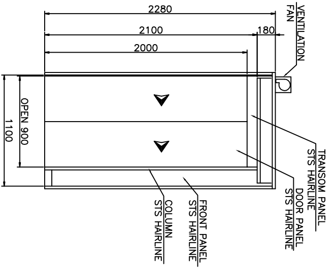
FRONT VIEW OF CABIN
