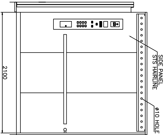
SIDE VIEW OF CABIN
