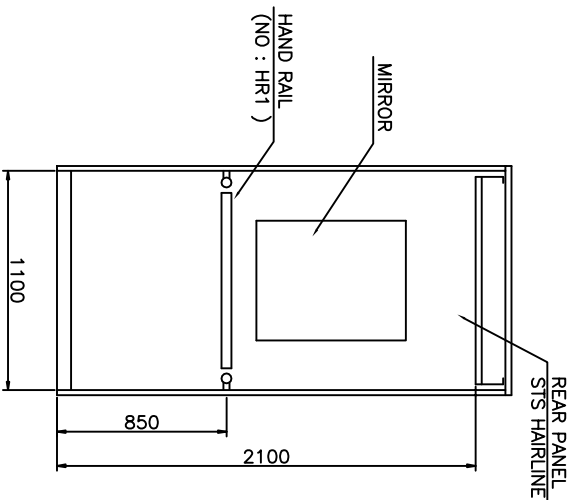
REAR VIEW OF CABIN
