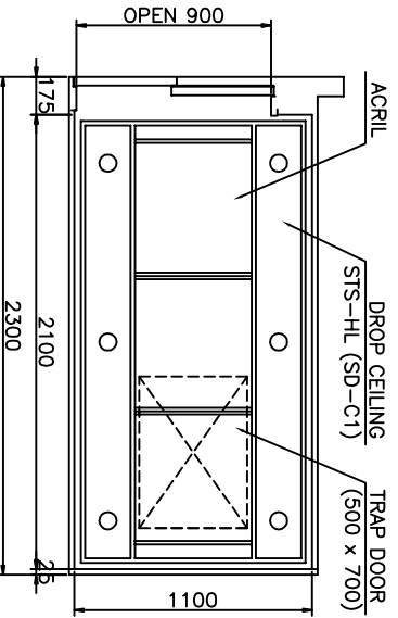
CEILING VIEW
