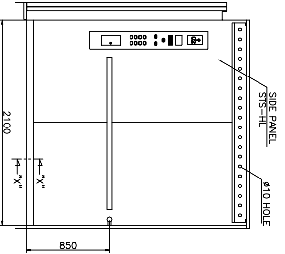
SIDE VIEW OF CABIN
