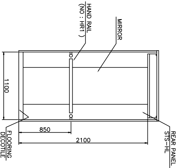
REAR VIEW OF CABIN
